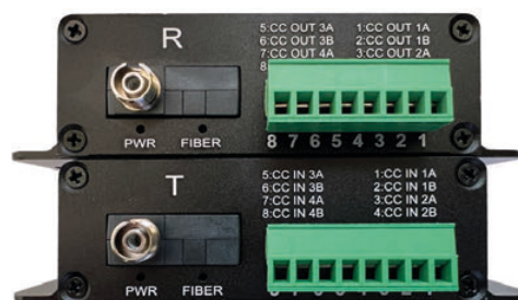
LOHD4CT transmitter+receiver
